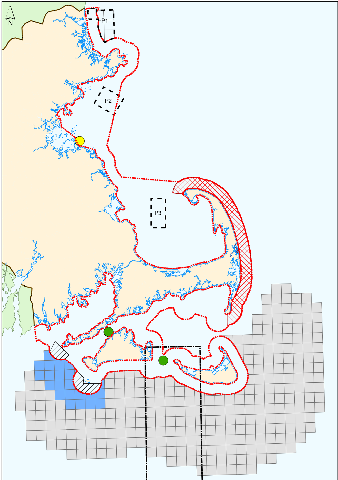
FIGURE 4-3 RENEWABLE ENERGY AREAS, INCLUDING ADJACENT FEDERAL WATERS
